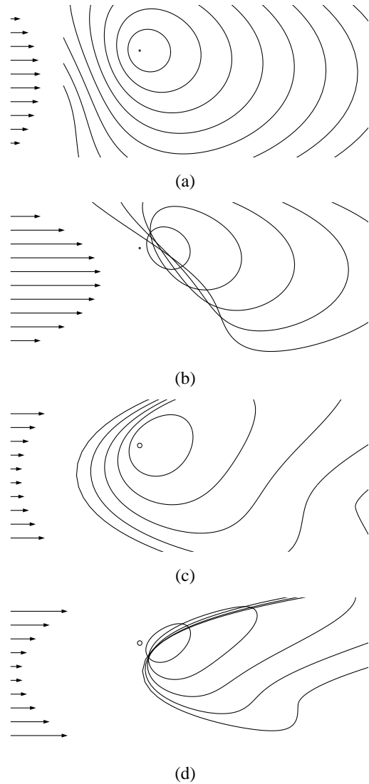
Fig. 5. Simulation of the diffusion of polluted material in various patterns of flow from the left to the right.
