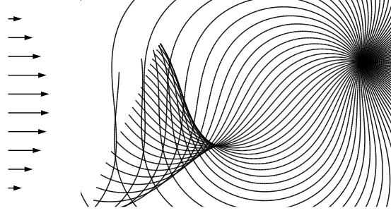
Fig. 4. Shortest paths for a boat in a flow field.
